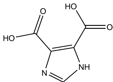
4,5-imidazoledicarboxylic acid
